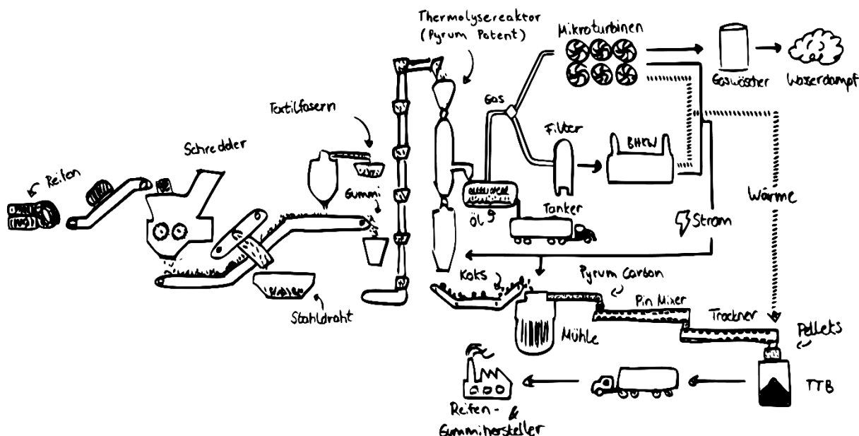
Fig. 3: Value chain of a Pyrum plant
